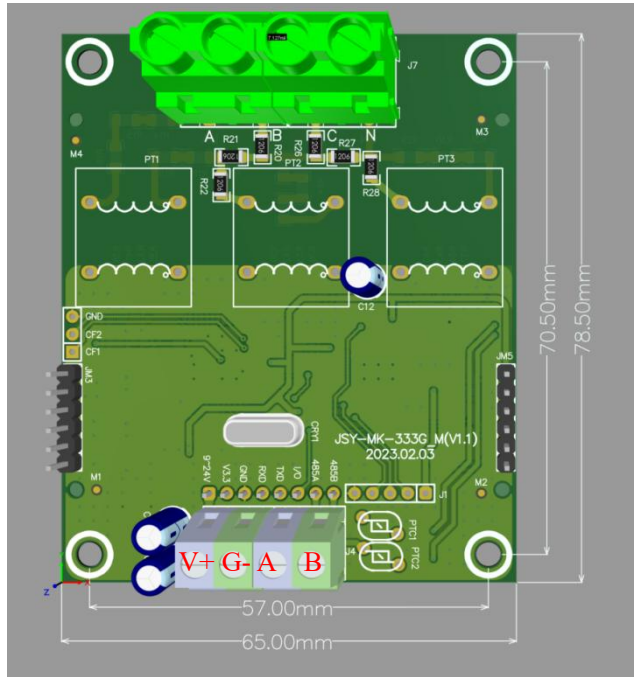
Figure 2.2.1 Product Form Factor and Functional Pinout
